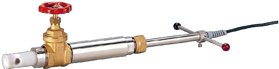
Fig. 14 Sensor mag-flux MIS 2/15 Flow-Probe
