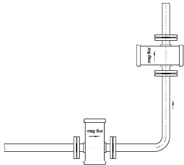
Fig. 2 Installation in horizontal and vertical pipelines
