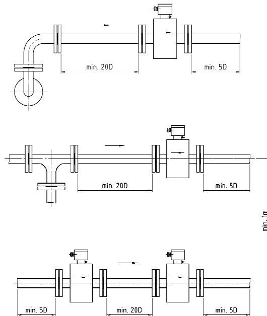
Fig. 5 Installation between tees, valves and pumps
