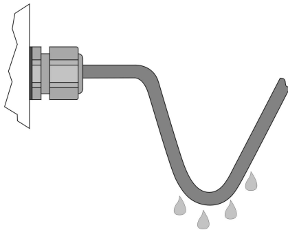
Fig 4.10 Installing the cables in front of the cable glands (loop)
