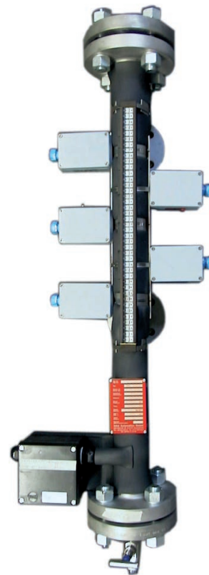
fig.3: ITA-3 with heating jacket and NI-Ex Switch
