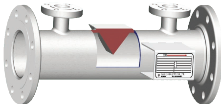
fig.2: Wedge Tube
