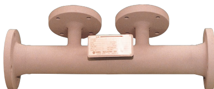
fig.3: Venturi with flanged process connection
