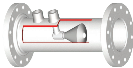
fig.4: V-Cone Flowmeter
