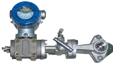
fig.1: Integral Orifice
