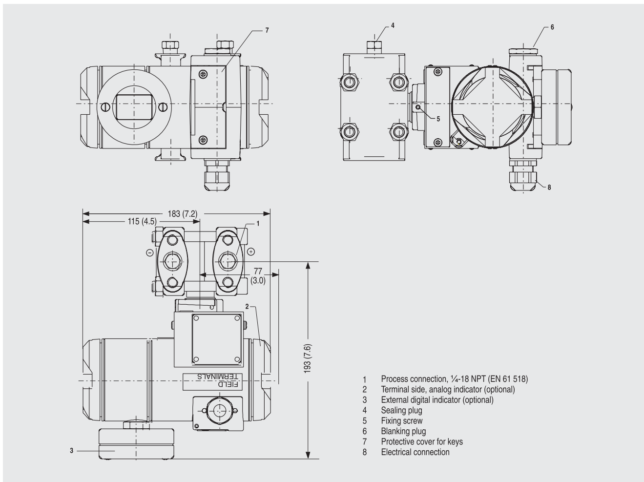
SITRANS P pressure transmitters, DS III FF series for differential pressure and flow, with digital indicator beside control keys, dimensions in mm (inch)
