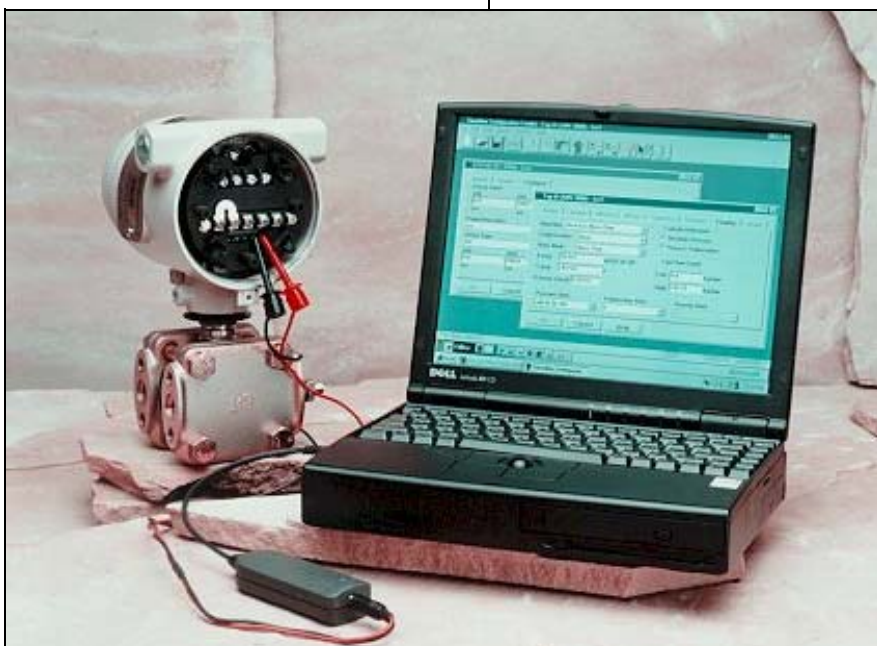
Figure 1 —SMV 3000 Smart Multivariable Flow Transmitter with SCT 3000 Smart Configuration Toolkit. The SMV 3000 measures differential pressure, static pressure and process temperature, and dynamically calculates mass or volumetric flow rate based on these measurements.
