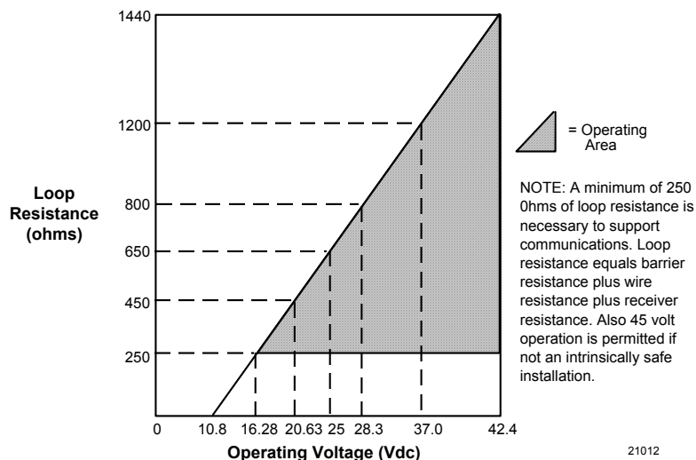
Figure 7 —Supply Voltage and Loop Resistance Chart.
