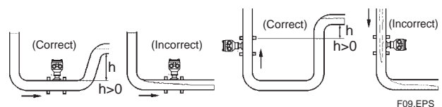
Mounting Positions
