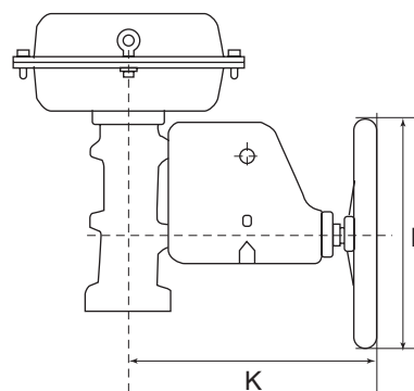
Figure 19 Side hand wheel
