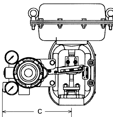
Figure 18 AVP positioner mounted
