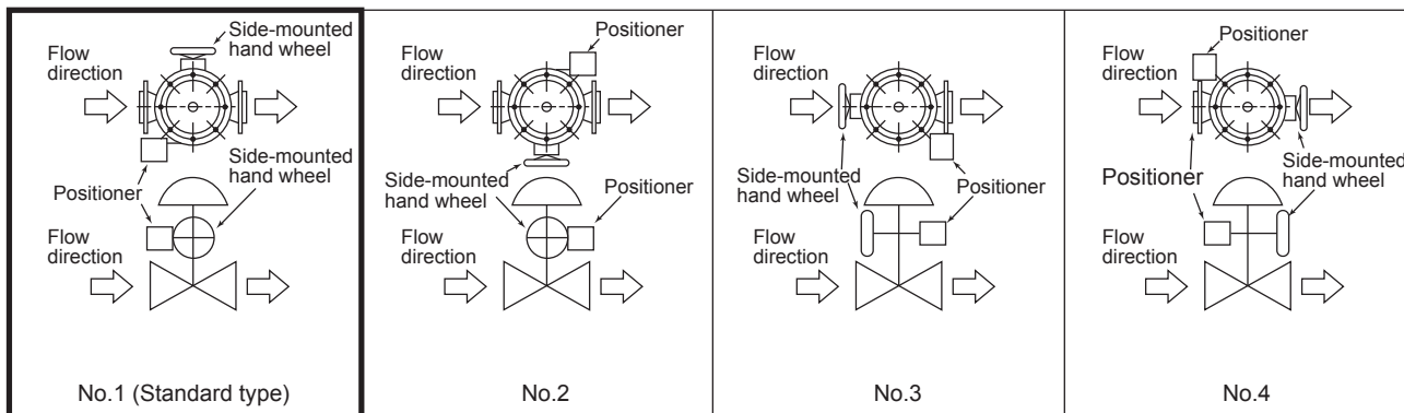
Figure 5 Actuator orientation
