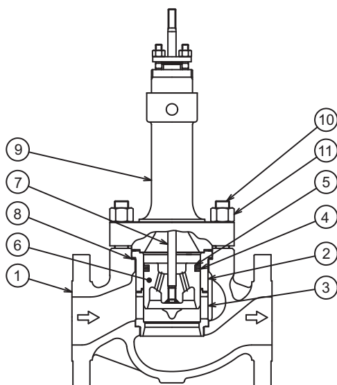
Figure 1-2 Model ACP structure drawing (temperature range: +230 to +360°C)
