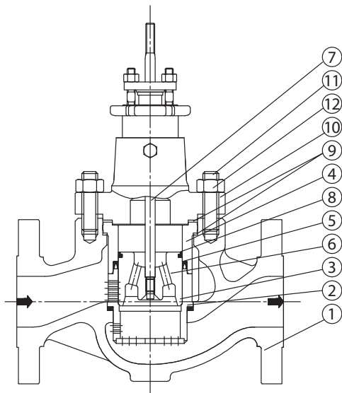
Figure 1-1 Model ACN structure drawing (temperature range: -196 to 230°C)
