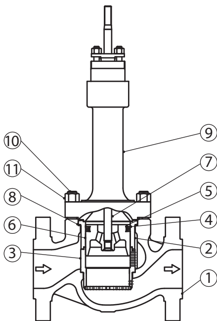
Figure 1-2 Model ACN structure drawing (temperature range: +230 to +360°C)
