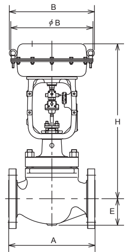
Figure 4 Face-to-face and other dimensions
