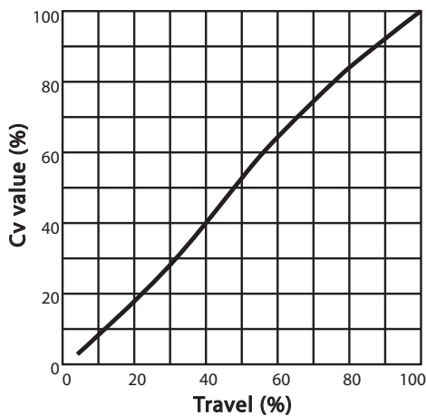
Figure 2 Flow characteristics
