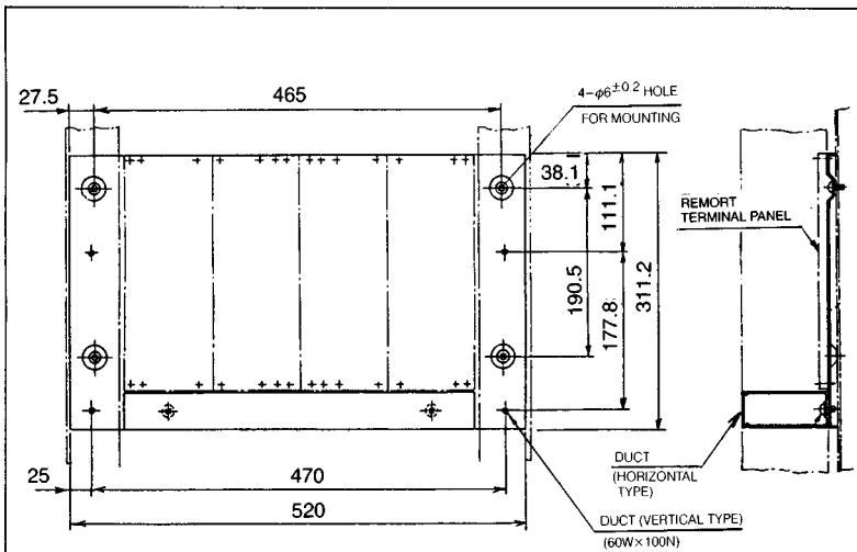
Fig. 13 Terminal Panel Supporter (J-TPX10)
