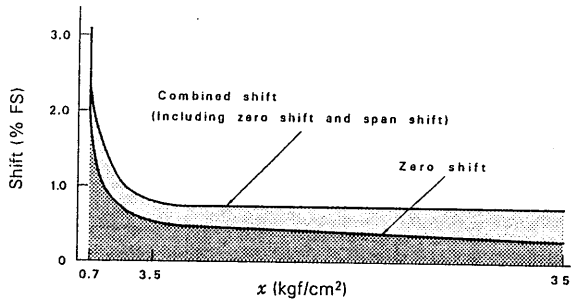
Fig. 3 Range and temperature effect (55 °C change)
