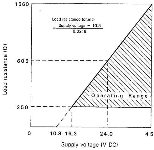
Fig.1 Supply voltage vs load resistance characteristics
