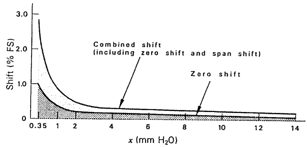
Fig. 4 Range and static pressure effect (70 kgf / cm² change)
