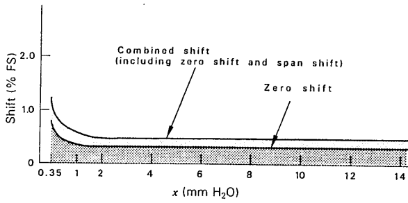
Fig. 3 Range and temperature effect (55 °C change)
