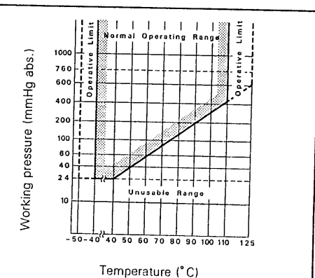
Fig. 2 Working pressure and temperature of wetted-parts section
