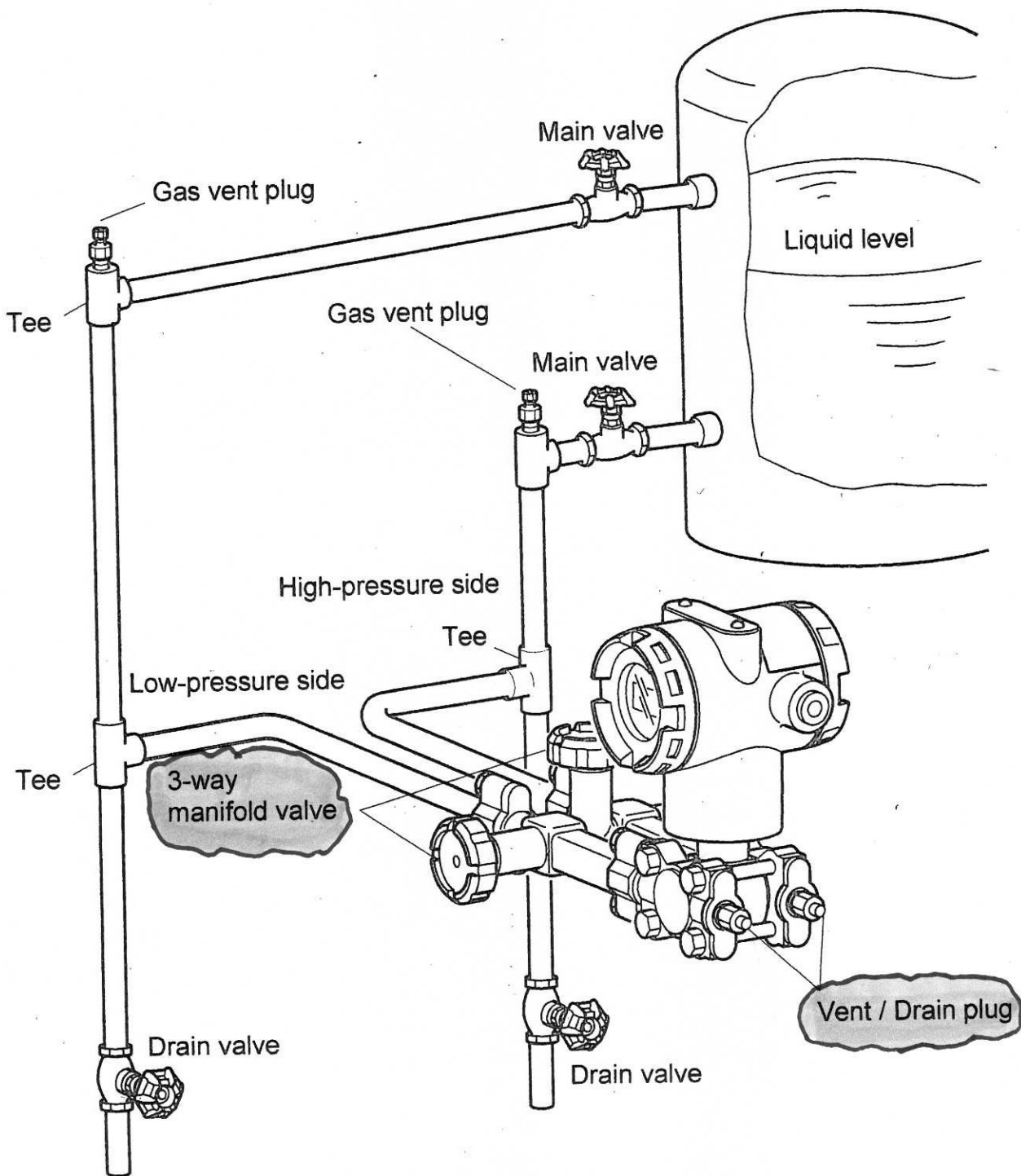
Figure 4-15 Closed Tank -- Piping (Dry-leg Sealing Example)
