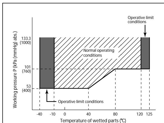
Figure 3 Working pressure and temperature of wetted parts section (for oxygen and chlorine models)
