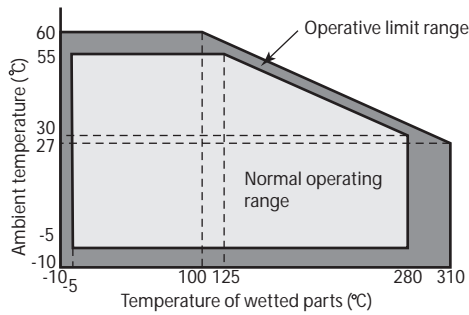
Figure 7 Ambient temperature and temperature of wetted parts section (for high temperature and vacuum 4, 5 m)
