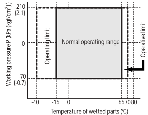
Figure 3 Working pressure and temperature of wetted parts section (for model STD910 regular type)
