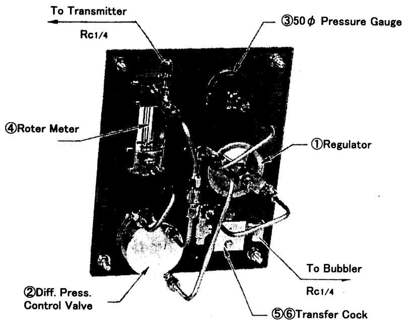
Air Purge Sets S Type with Transfer Cock
