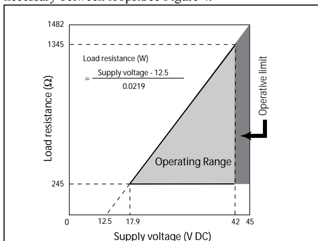
Figure 4 Supply voltage vs. load resistance characteristics
