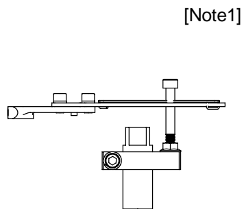
Fig.1 Feedback lever assembly
