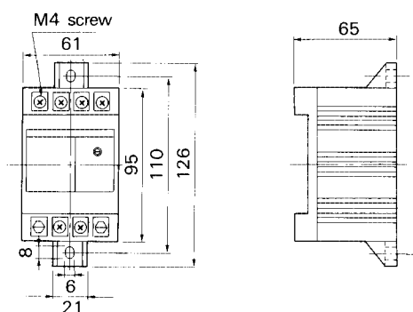
Figure 3. Power supply unit (for 1 to 5V DC input, YMW-080)
