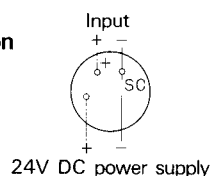
Figure 2. Dimension and terminal connection drawings of YMW
