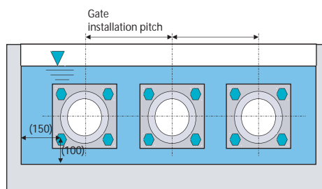
Figure 14 Installation pitch
