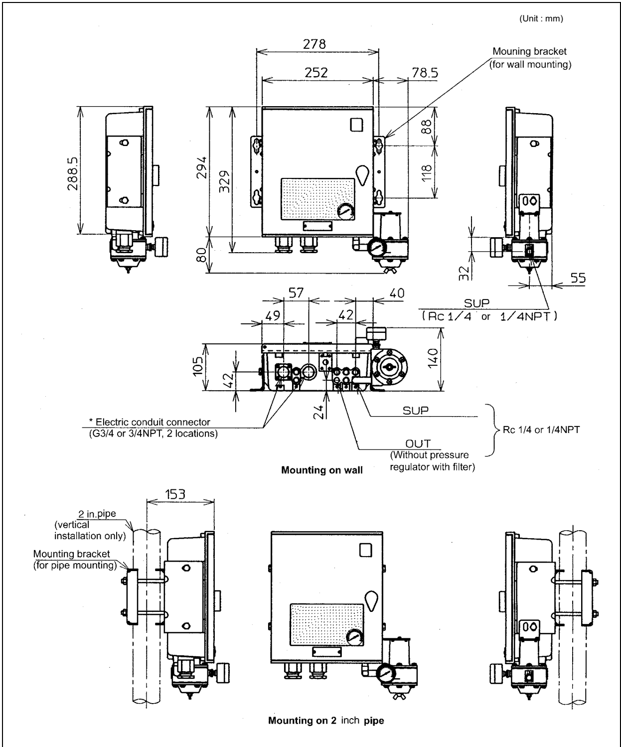
Figure 3. External Dimensions
