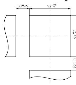
Individual mounting
