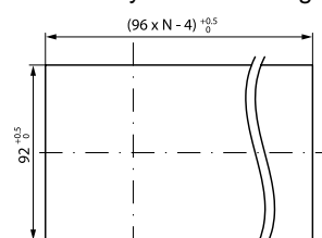
Side-by-side mounting
