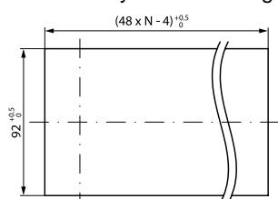
Side-by-side mounting
