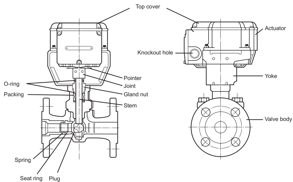
Figure 2. Parts identification
