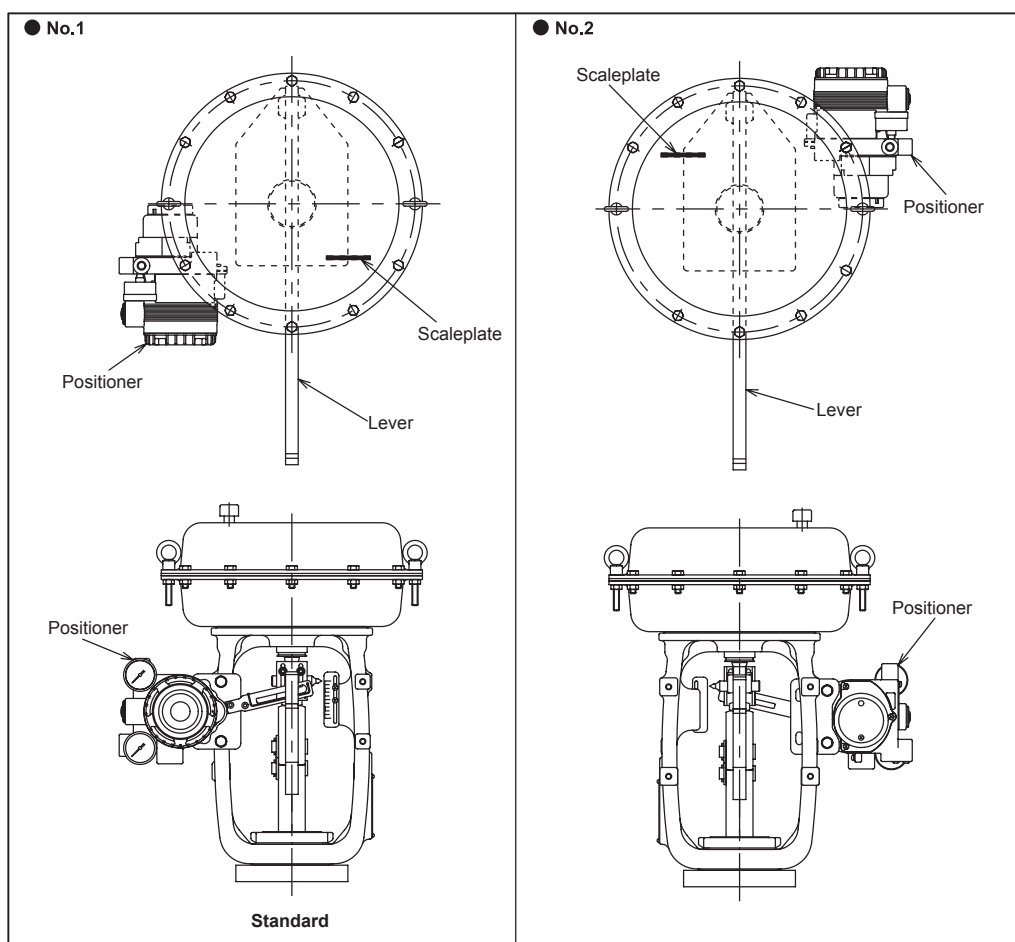
Figure 3 Actuator orientation
