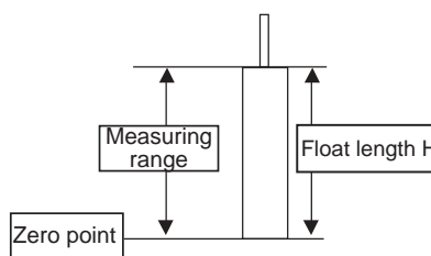
Figure 7 Appropriate way of adjustment: Set float bottom at zero point
