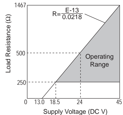
Figure 3 Power supply voltage / load resistance
